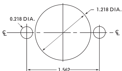
RECOMMENDED CHASSIS CUT-OUT
